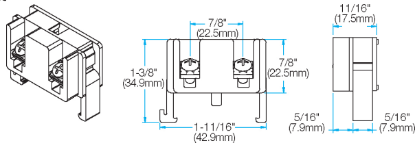
Logic Reed Contact Block
