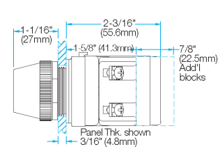
Dual Input Pilot Light Operator
