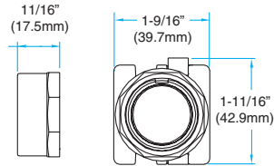
Momentary Guarded Flush Cap
