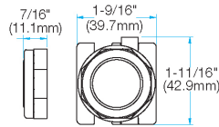
Momentary Flush Cap
