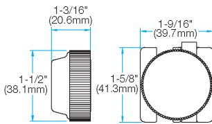
Momentary Standard Rubber Boot
