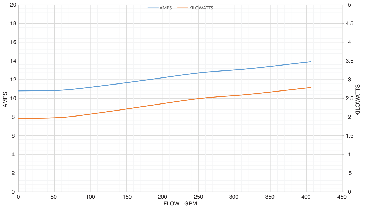
PERFORMANCE CURVE
