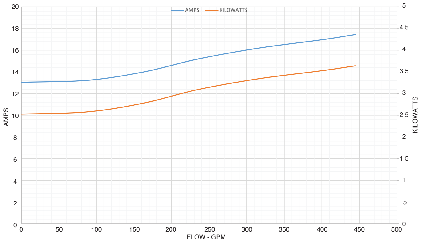
PERFORMANCE CURVE
